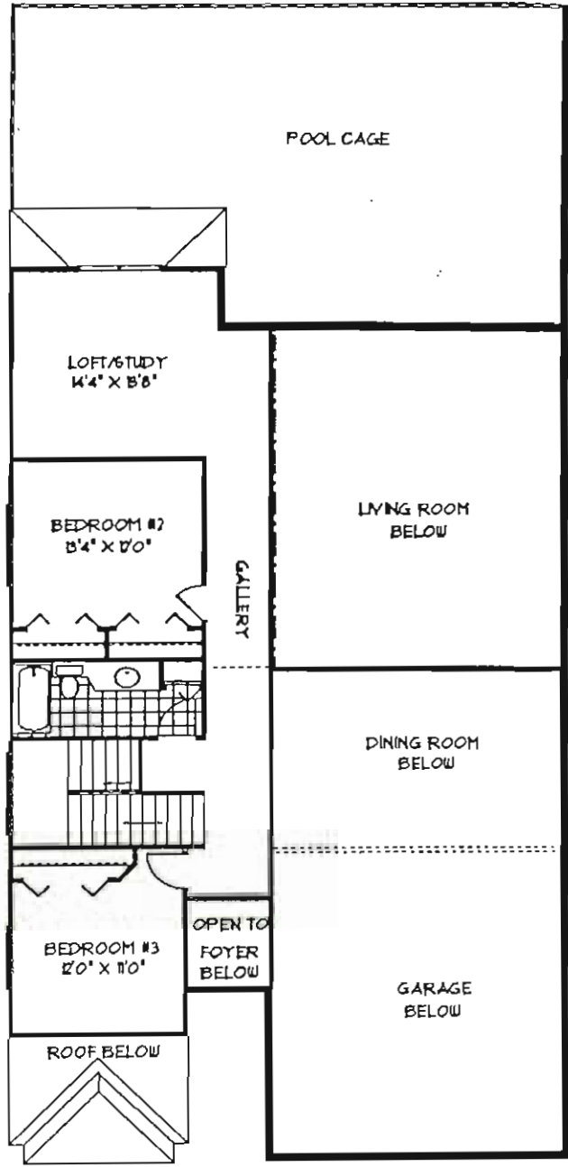
2ND FLOOR
