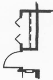
SINGLE DOOR AT MASTER SUITE
