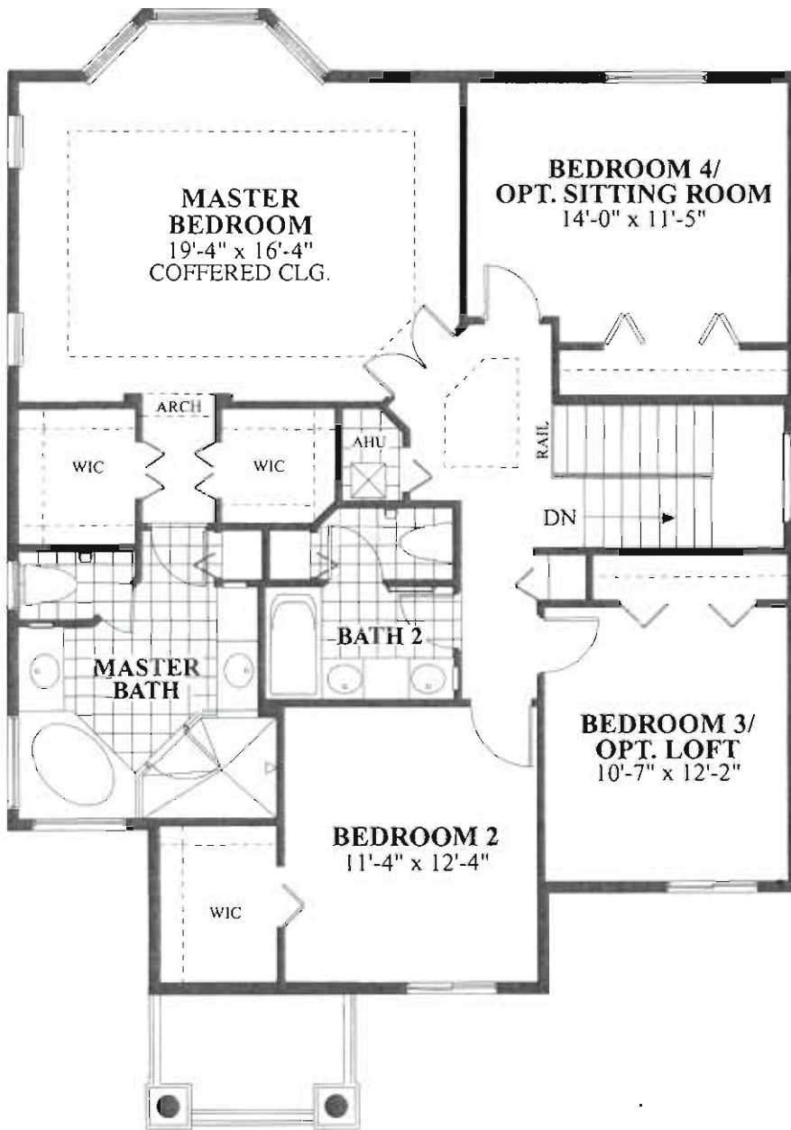
SECOND FLOOR 8' 4" CEILING HGT. UNLESS OTHERWISE NOTED ELEVATION A
