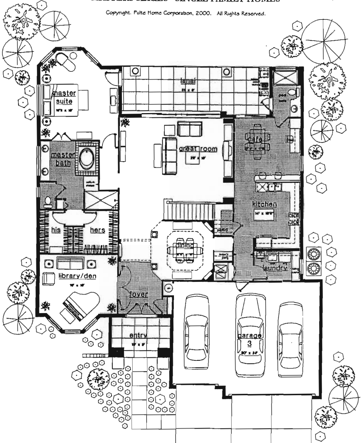
FIRST FLOOR TURNBERRY 3400
