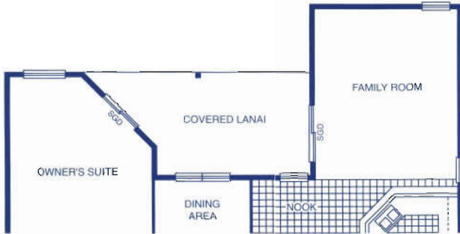
#6 26' X 12' COVERED LANAI W/EXPANDED OWNER'S SUITE
