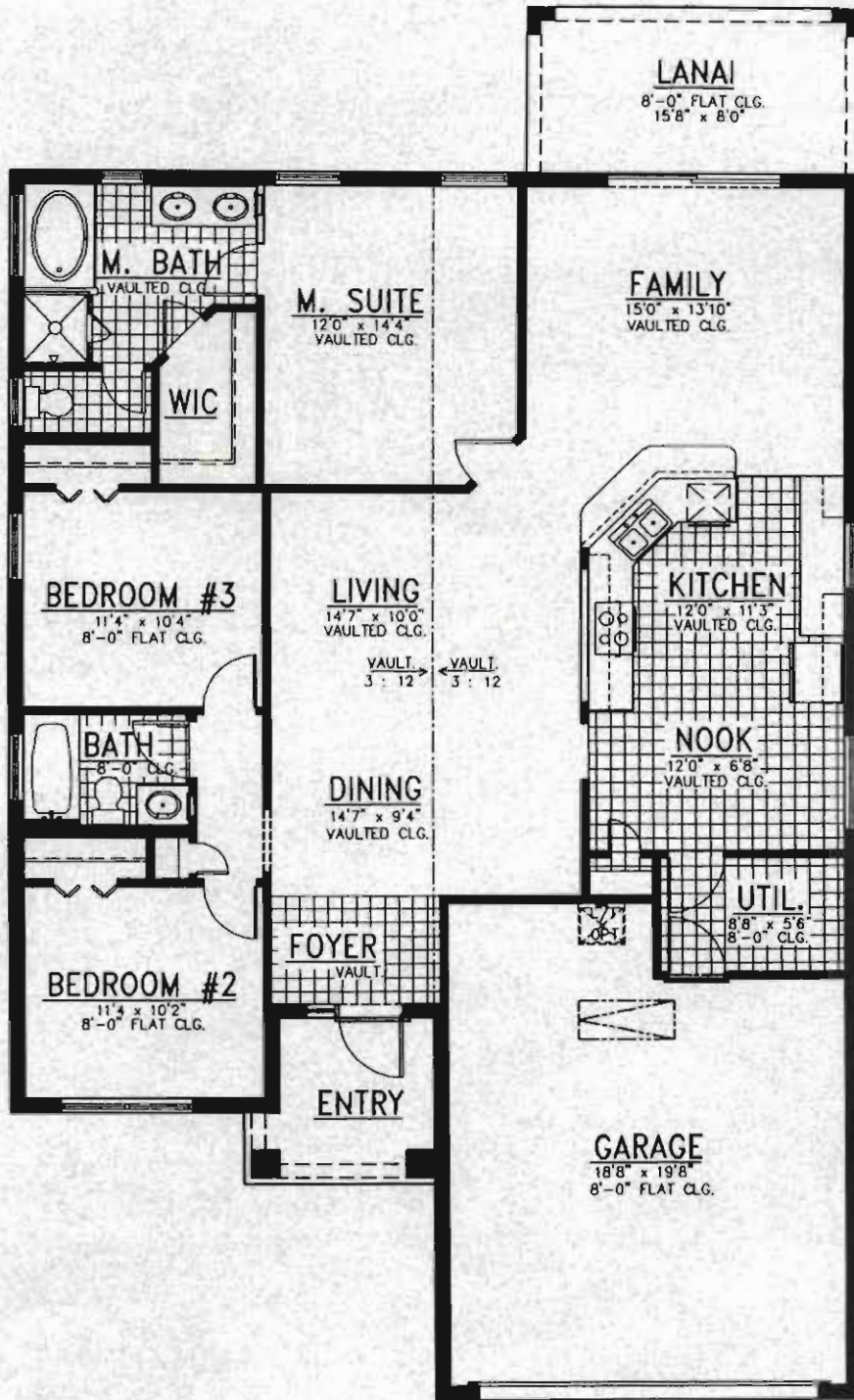
FLOOR PLAN
