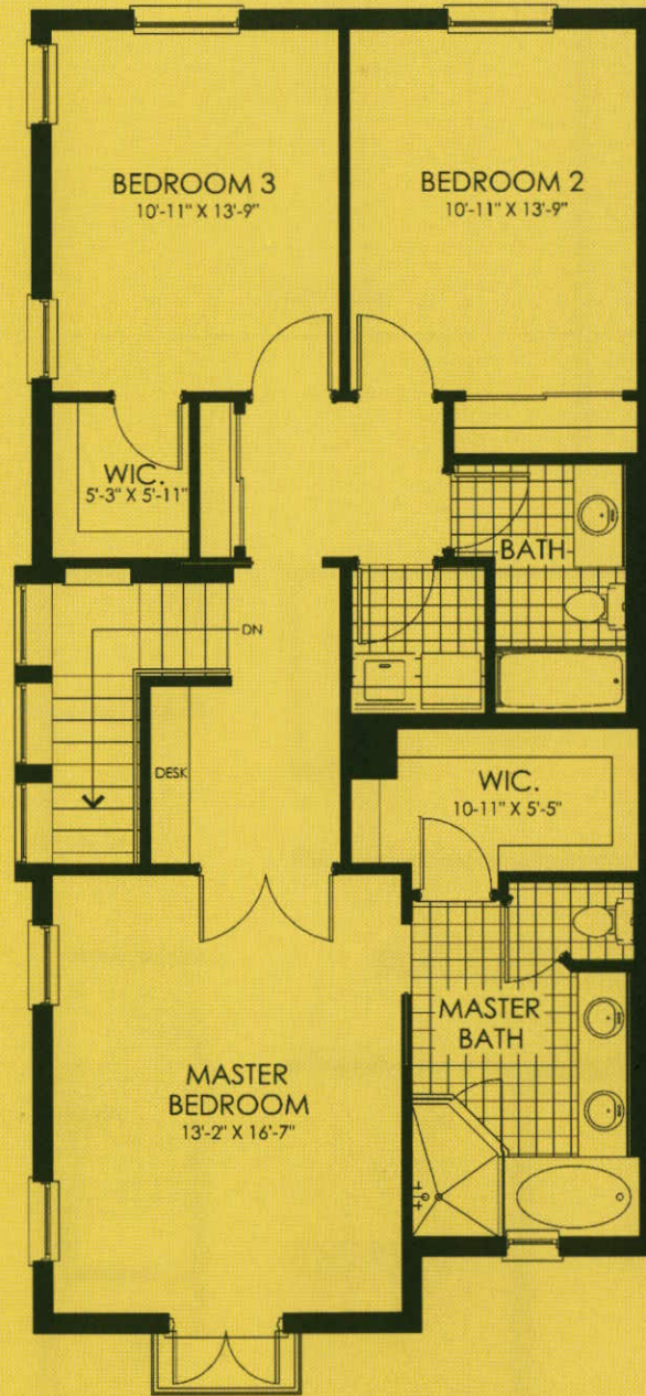
SECOND FLOOR
